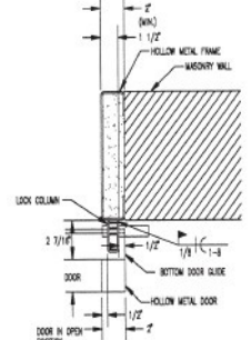
DETAIL B – VERTICAL LOCK JAMB BAR
